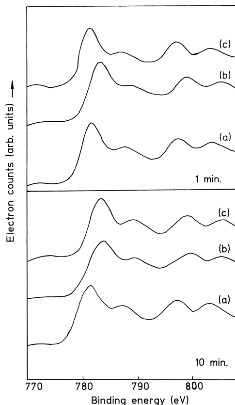
Fig. 7. XP (Co 2p) spectra of spent catalysts after 1 min \text{Ar}^+ and 10 min \text{Ar}^+ sputter etching (a) \text{CoAl}_{2.0}:1\text{-HT(}^{\text{LS}}) , (b) \text{CoAl}_{2.5}:1\text{-HT(}^{\text{LS}}) , (c) \text{CoAl}_{3.0}:1\text{-HT(}^{\text{LS}}) .
