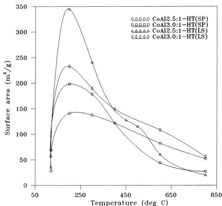
Fig. 2. Variation of surface area with calcination temperature for Co–Al HT-like compounds.
