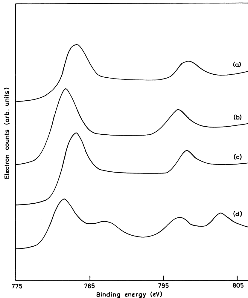
Fig. 6. XP (Co 2p) spectra of spent catalysts (a) CoAl 2 O 3 :1-HT(LS), (b) CoAl 2 O 3 :1-HT(LS), (c) CoAl 3 O 8 :1-HT(LS), (d) CoAl 2 O 4 .
